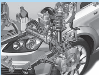
MacPherson strut front suspension.
